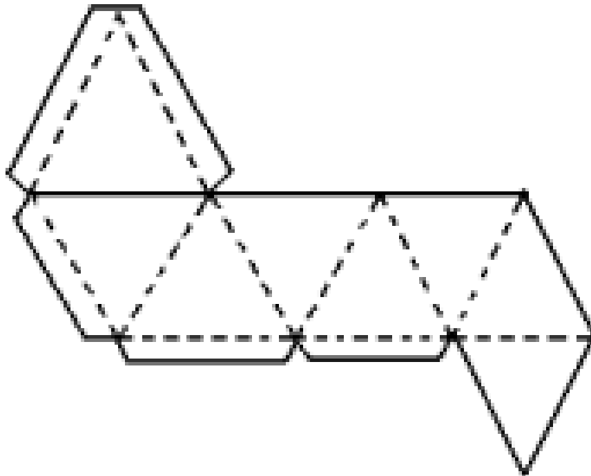
Octaedro Regular
