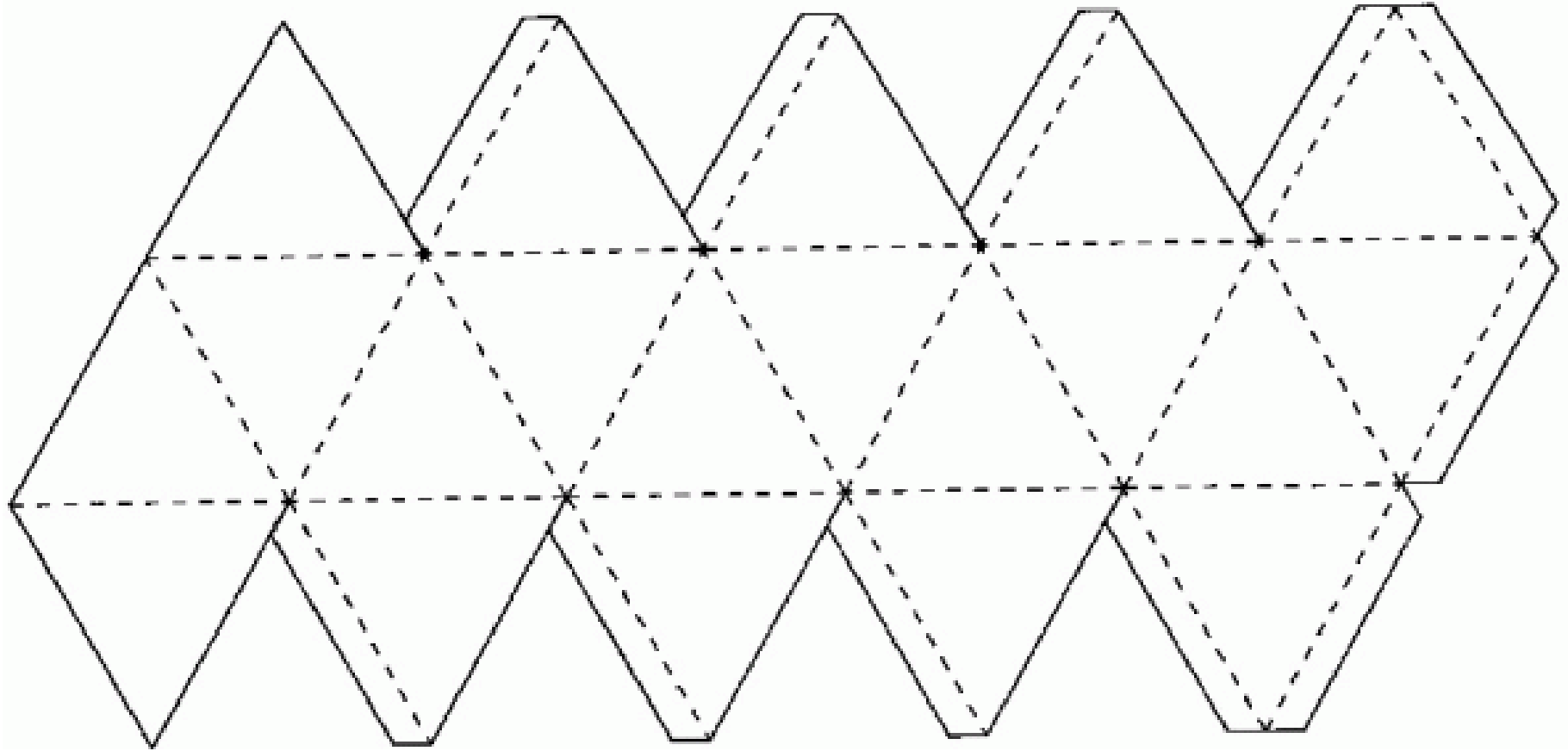
Icosaedro regular
